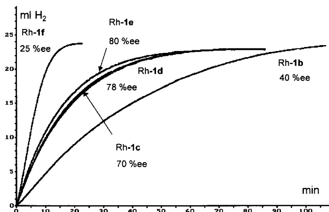
Figure 1 Asymmetric hydrogenation of ItMe 2 under standard conditions (15.0 ml of MeOH, 25°C, 0.1 MPa total pressure, 0.01 mmol of precatalyst, 1.0 mmol substrate)
